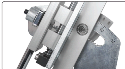
▲ High resolution lie angle scale with rack and pinion for lie angle control
