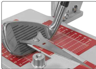
▲ Face angle and leading edge alignment apron improves lie measurement accuracy
