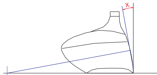
▲ Loft angle on woods is measured at half the club face height.
