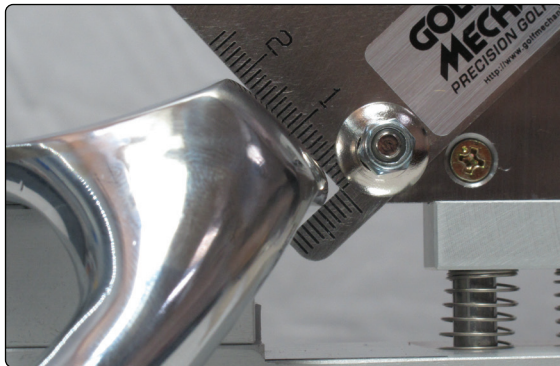
▲ Bounce angle, sole width and edge height measured in one step.
