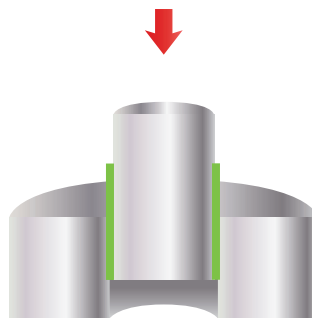
▲ Bonded slip fit
