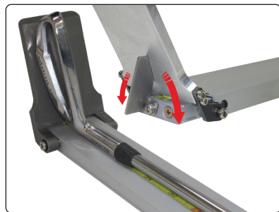
▲ Back stop to lock tipping plate to 60°; for measure clubs in sanctioned events
