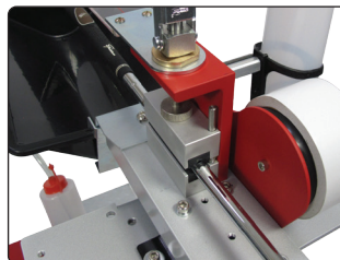
▲ Adjustable pressure speed clamp with centred rubber V-jaws
