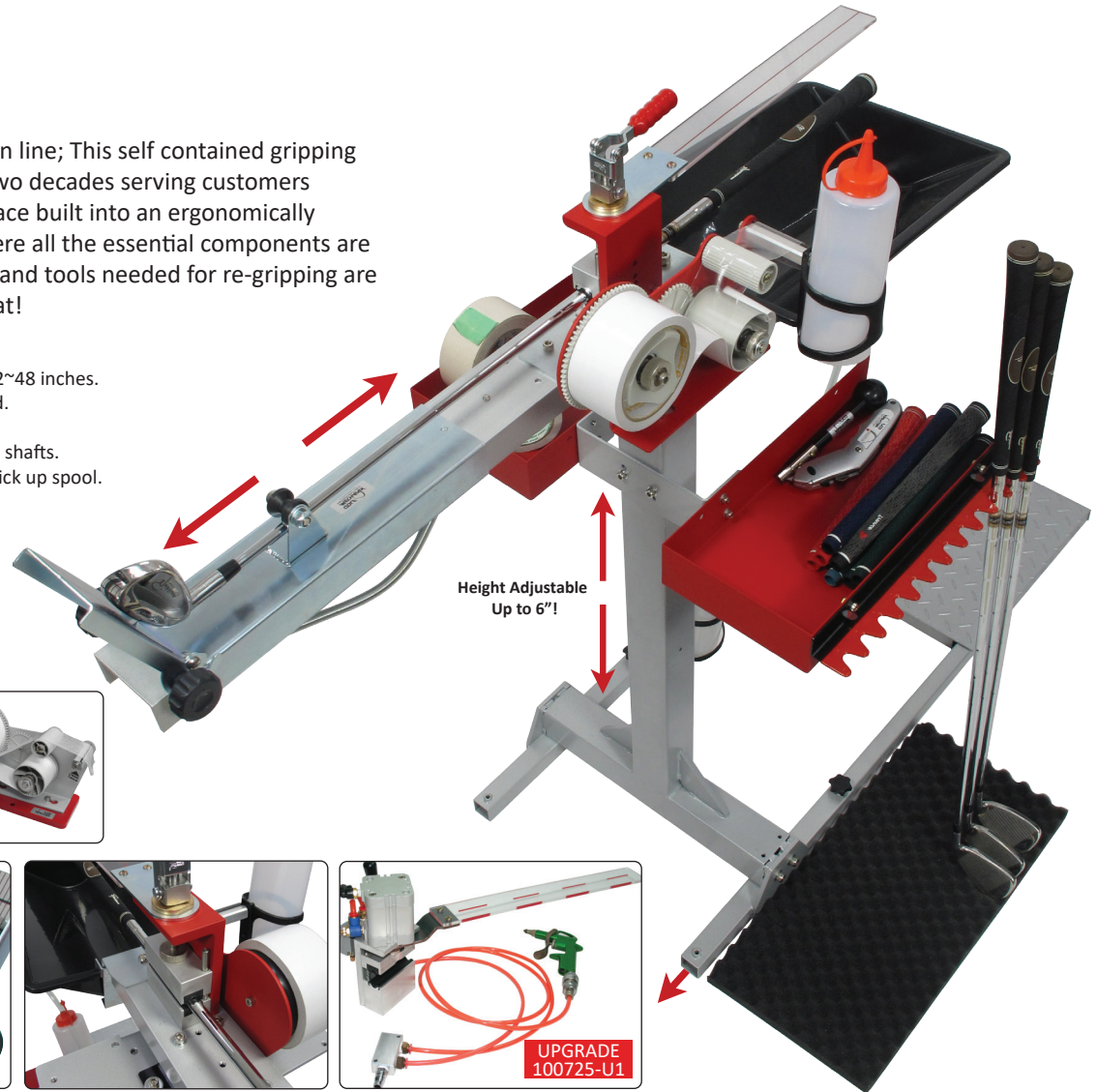
▲ Adjustable pressure speed clamp with centred rubber V-jaws
