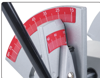
▲ High visibility direct reading full scale lie and loft protractor with a resolution of better than 1°
