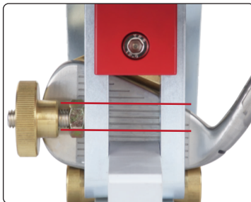
▲ Toe Stop prevents slippage when iron is positioned and secured in the gauge. Slot provides clear sighting of grooves to aid in locating the iron in the correct lie position.
