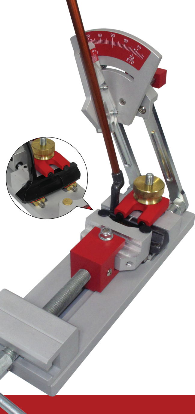
▲ Self levelling, interchangeable kinematic soling pads provide maximum support.
