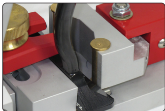
▲ Putter pinned down by the reduced interference, soft clawed back clamp with the least force.
