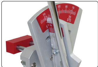
▲ Protractor adequate for most fitting alteration and accurate to 1 degree
