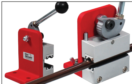
▲ Ratchet provides a reliable fuss free convenience.
